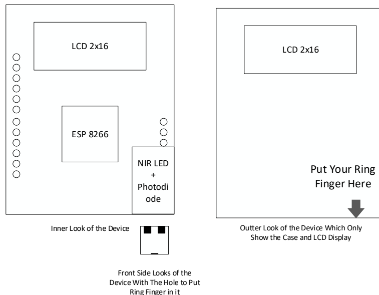
Figure 2. Device's Design
