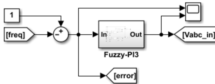
Figure 3. Block Diagram of ELC Control in Simulink
